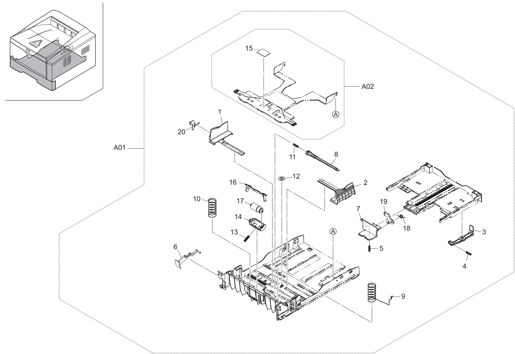
FIG. 3 Paper Cassette
